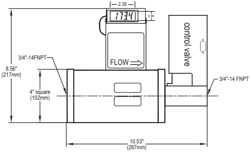
GFC77 MASS FLOW CONTROLLER
